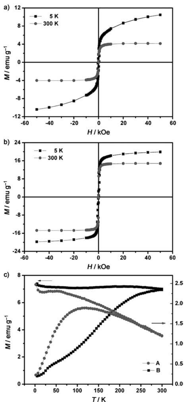
Figure 4. a,b) Field-dependent magnetization curves (at T=5 and 300 K) of sample A (a) and B (b). c) ZFC-FC magnetization curves ( H=100 Oe) of A and B.
